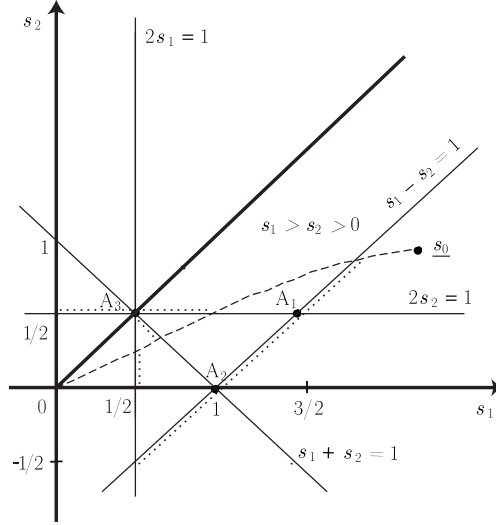
FIGURE 2.2.2. Case A singular hyperplanes
