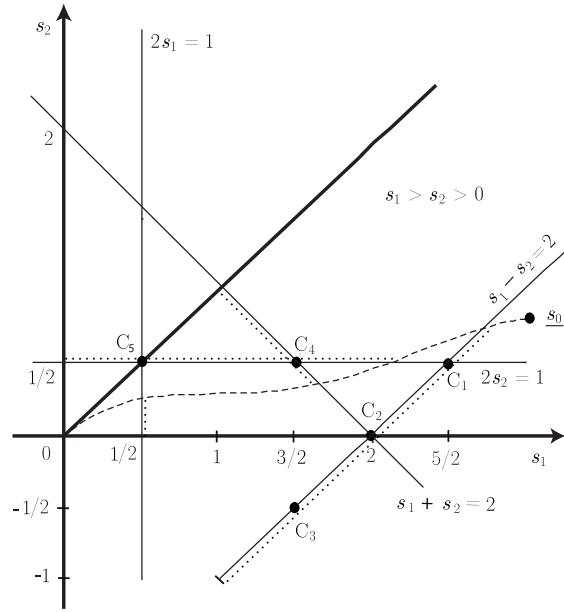
FIGURE 2.4.2. Case C singular hyperplanes
