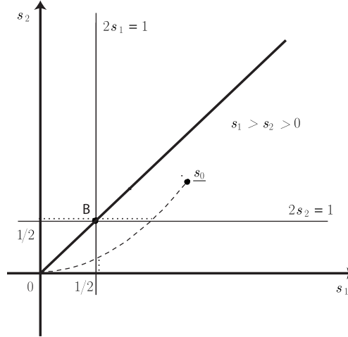
FIGURE 2.3.2. Case B singular hyperplanes
